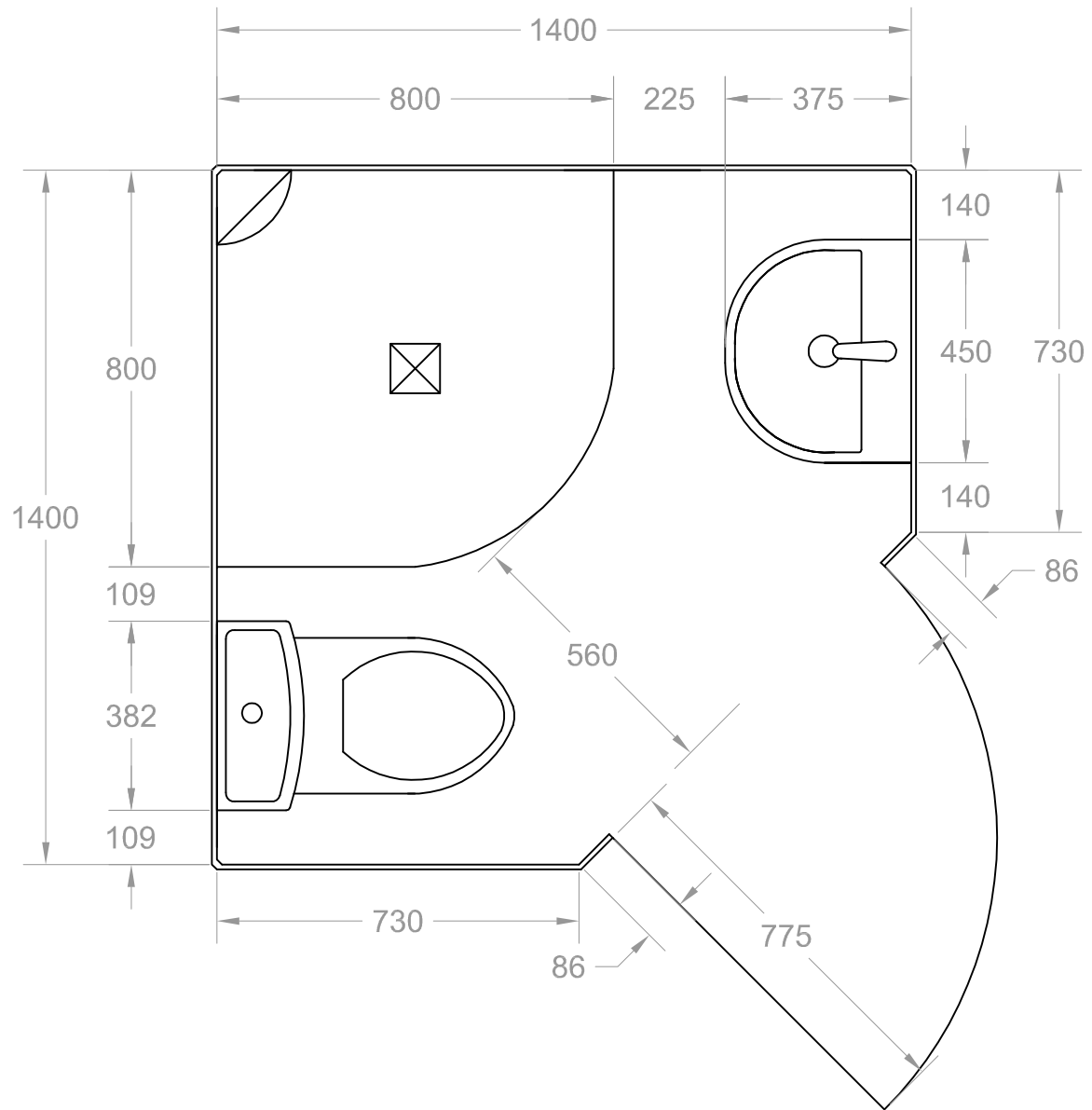
SIGNA BATHROOM POD 1400X1400 CORNER UNIT
